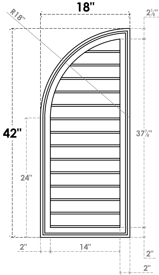
FRONT
